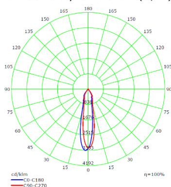
Luminous Intensity Distribution Curve(cd/klm)
