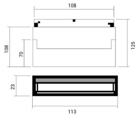
SH-MFA6-2M
